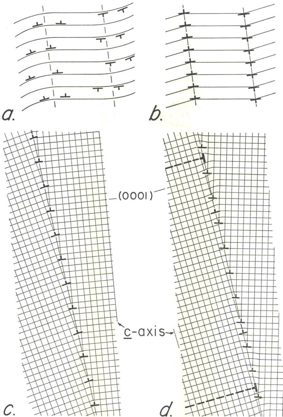
FIG. 6.—Dislocation models of band boundaries. a , simple deformation band showing edge dislocations of opposite sign accumulated in slip planes at opposite boundaries of a band. b , polygonized band boundary, showing dislocations redistributed into two walls of opposite sign at the boundaries ( a and b after Cottrell, 1953, p. 166). c , model of a symmetrical kink boundary in quartz viewed parallel to the dislocation lines. Tilt is approximately 7^\circ on each side of boundary. d , model of an asymmetrical band boundary in quartz, viewed along the dislocation lines. Tilt is approximately 2^\circ on left side of the boundary and 12^\circ on right. Basal edge dislocations introduce extra prism planes on each side of boundary, and prismatic edge dislocations introduce extra basal planes (heavy broken lines) on side with smaller tilt. (In c and d distortions of the prism planes in the neighborhood of basal edge dislocations are omitted for simplicity.) Basal and prismatic dislocation lines are assumed to be normal to the plane of the figure.
